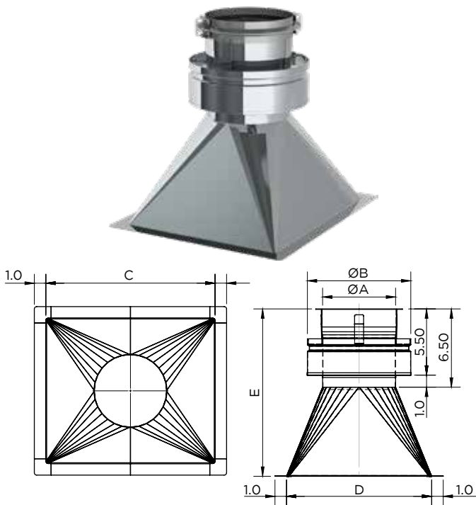
Transition to Round - Start / DWFLØ-STR
