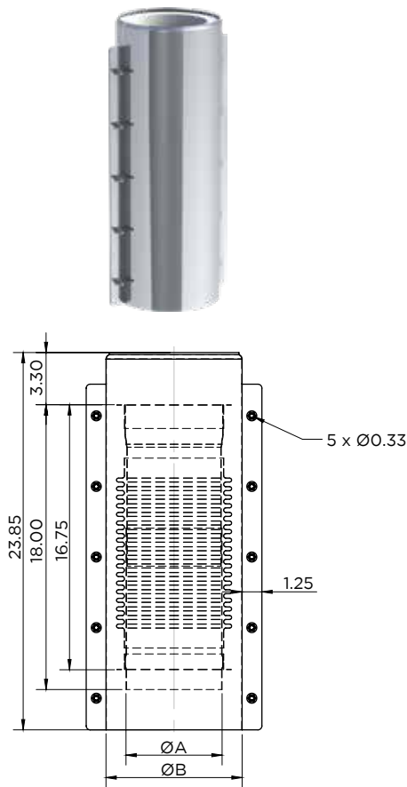
18" Lined Bellows Length / DWFLØ-LBL
