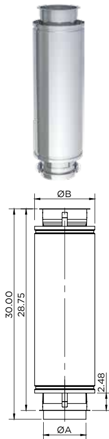
30" Fixed Length / DWFLØ-30L
