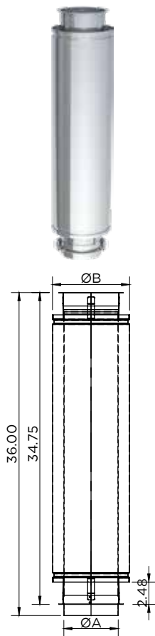
36" Fixed Length / DWFLØ-36L
