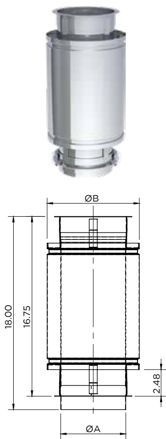
18" Fixed Length/ DWFLØ-18L
