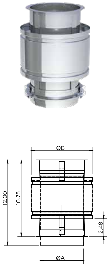
12" Fixed Length / DWFLØ-12L
