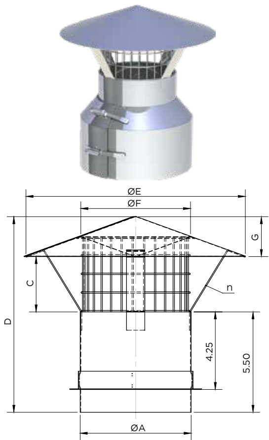
Stack Cap with Screen / DWFLØ-SCS
