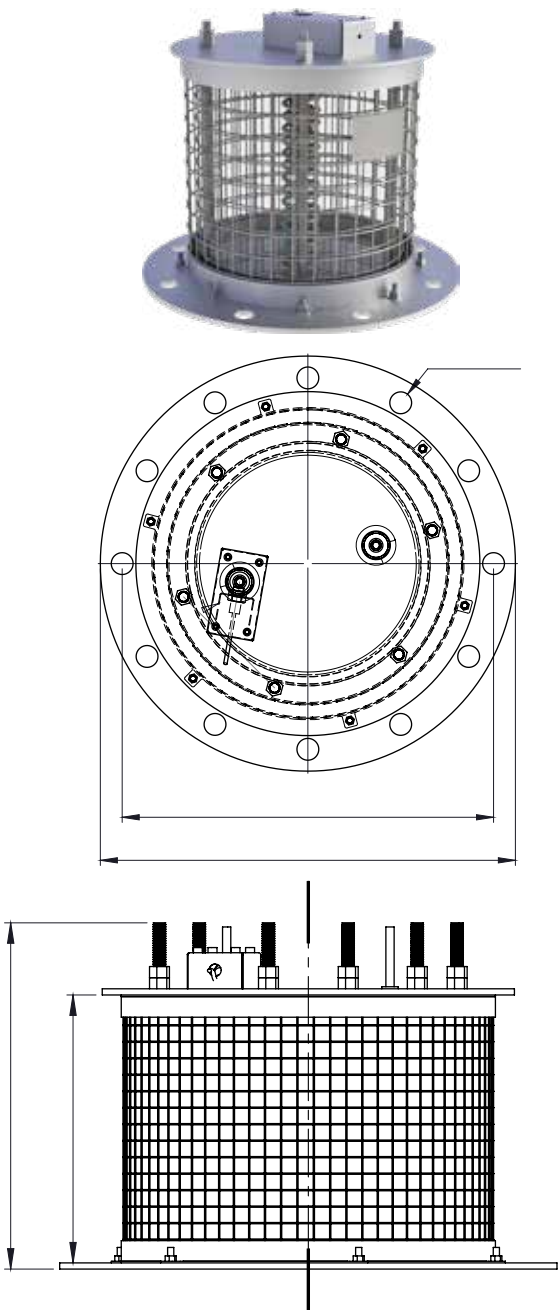
Flame Retardant Pressure Relive Valve / DWKLØ-PRVF
