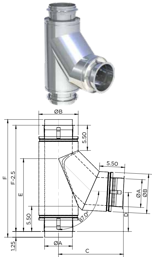
87° Grease Boot Tee / DWFLØ-90GBT
