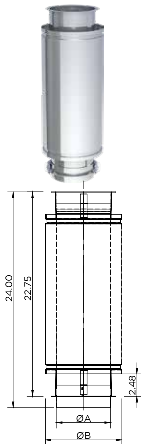
24" Fixed Length / DWFLØ-24L
