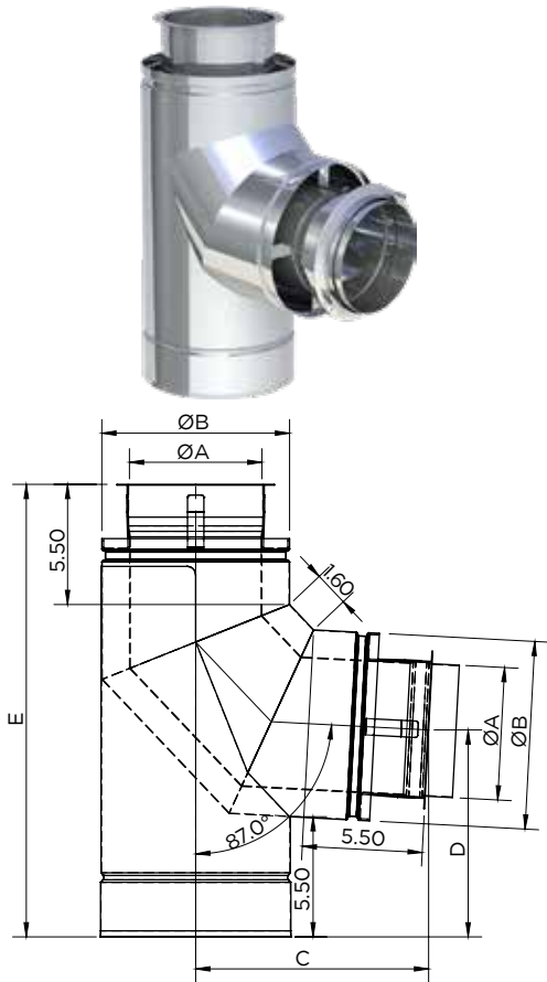
Elbow 87° with support leg / DWFLØ-87ES
