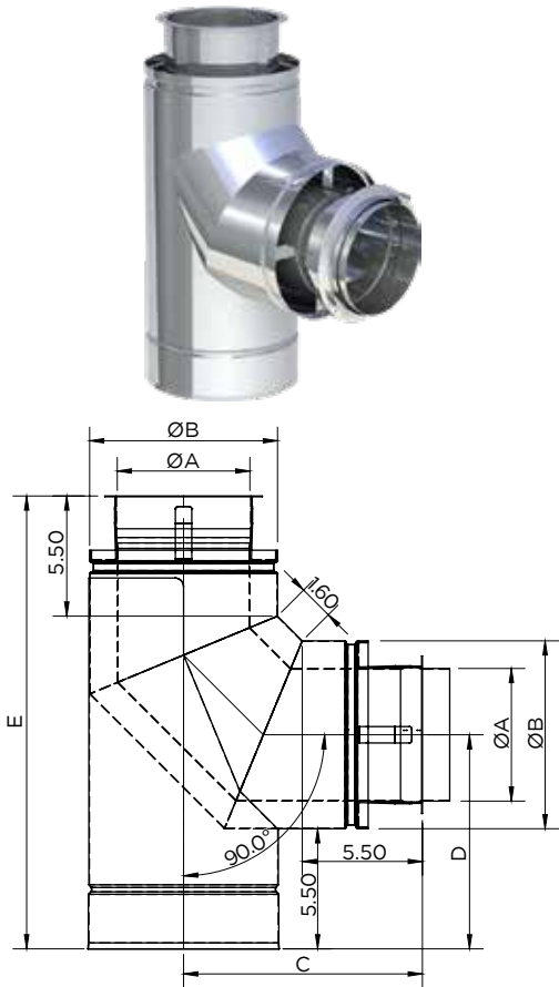
Elbow 90° with support leg / DWFLØ-90ES
