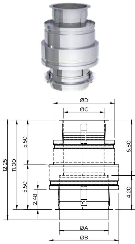
Stepped Reducer / DWFLØ-SR
