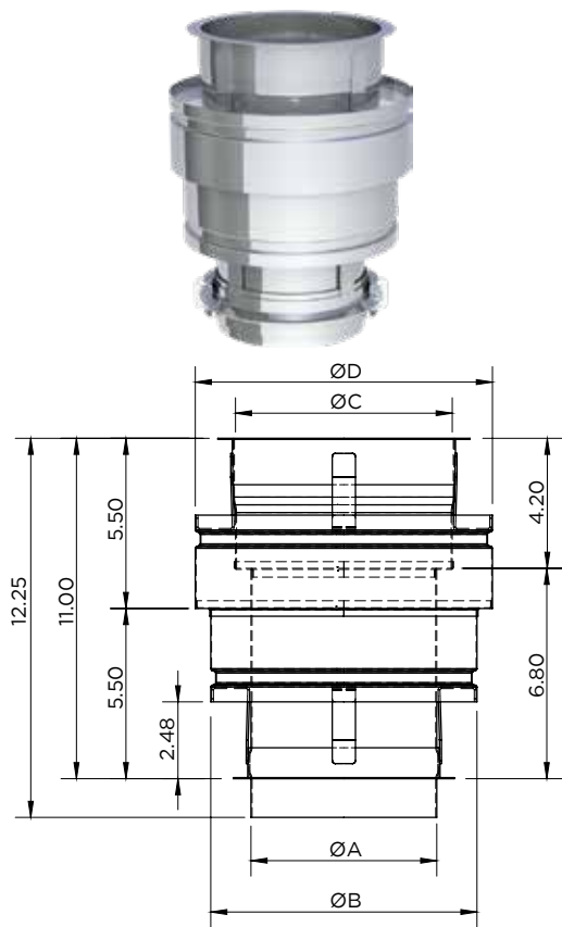
Stepped Increaser / DWFLØ-SI
