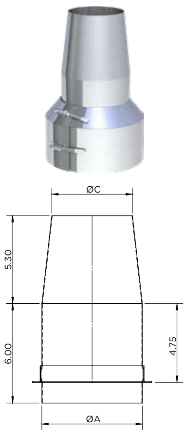
Exit Cone / DWFLØ-EC
