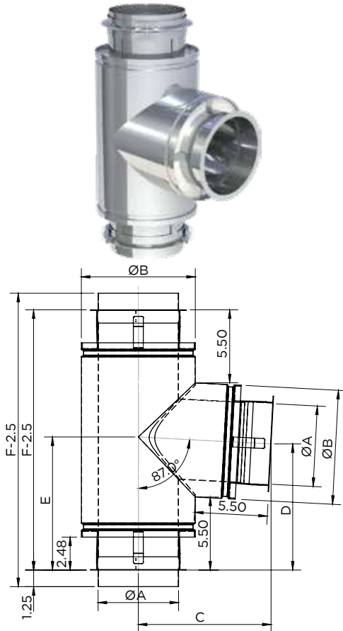
87° Grease Duct Tee / DWFLØ-87GT
