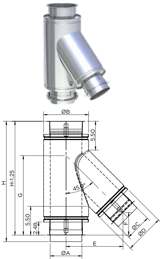
45° Reduction Tee / DWFLØ-45TØ
